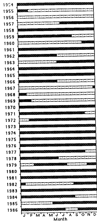
Figure 3.22 Wellstead Estuary. Reported opening and closing of the bar. ■ closed, ▨ open. (A. & J. Jury, pers. comm.)
