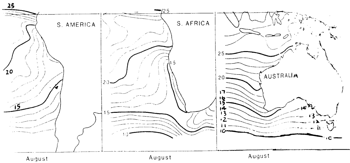
Winter (August) sea-surface temperature charts off the western coasts of South America, southern Africa and Australia (after Reynolds 1982).
