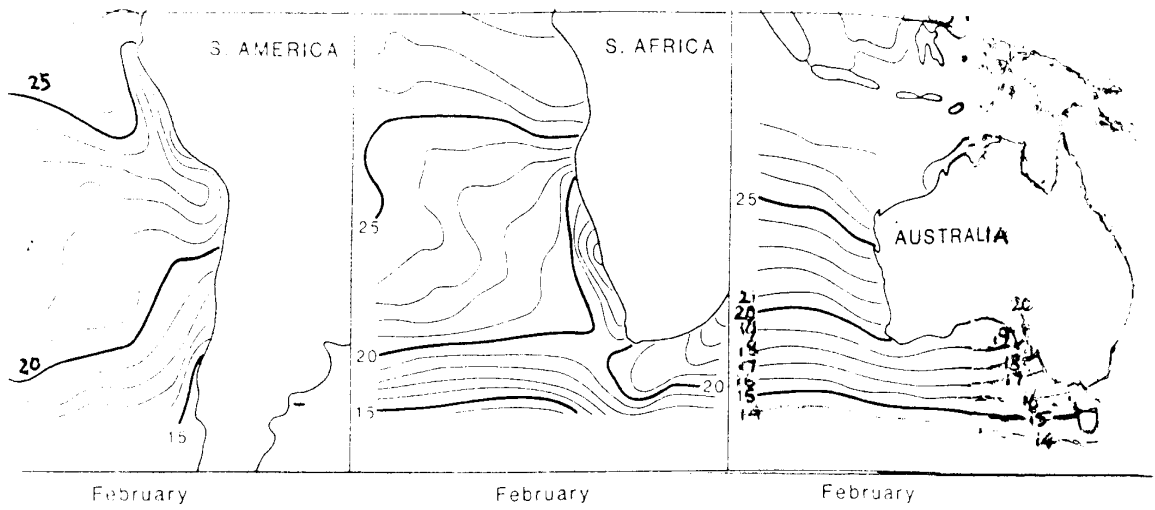
Summer (February) sea-surface temperature charts off the western coasts of South America, southern Africa and Australia (after Reynolds 1982).
