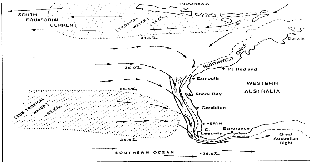
Figure 1 Schematic chart of the large-scale circulation in the eastern Indian Ocean. The Leeuwin Current is shown as the hatched area off Western Australia (From Pearce & Cresswell 1985).
