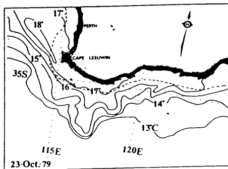
Fig. 4 Surface ocean temperature from FINS (1982).
