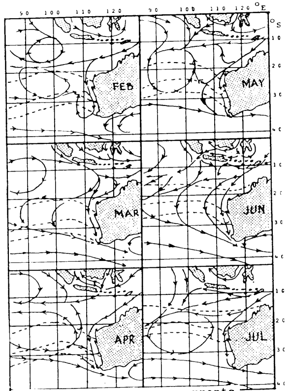
Fig. 5 Surface ocean currents from Robins (1975).
