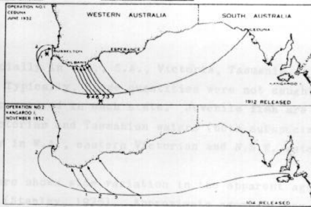
Migration of tagged fish from South Australia to Western Australia. Numbers denote recaptures from each locality.
