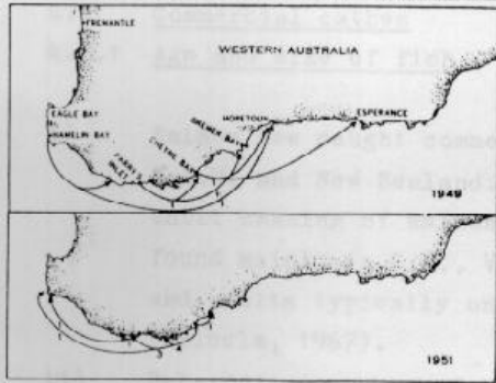
Movements of Australian salmon tagged in Western Australia. Top, post-spawning movements in 1949. Below, prespawning movements in 1951.
